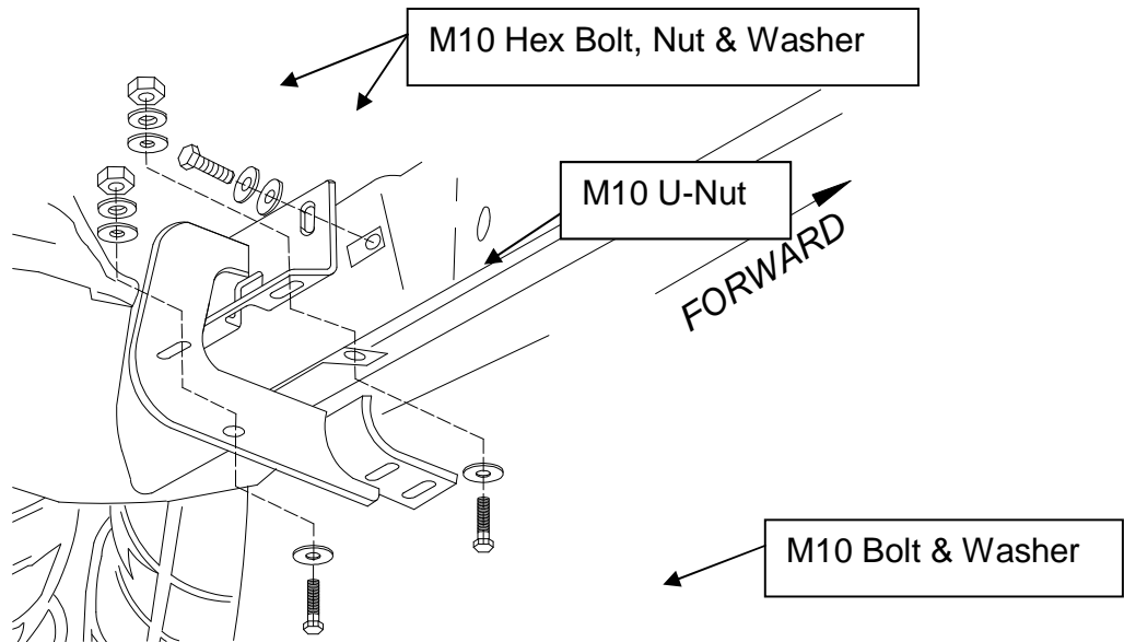
Figure 2. Driver Side – Rear Bracket
