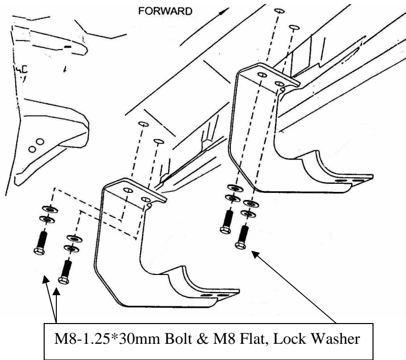
Figure 2. Passenger Side –Center & Rear Bracket
