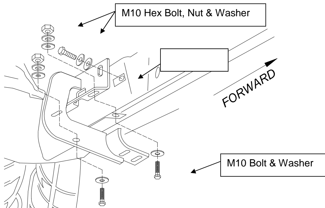
Figure 2. Driver Side – Rear Bracket
