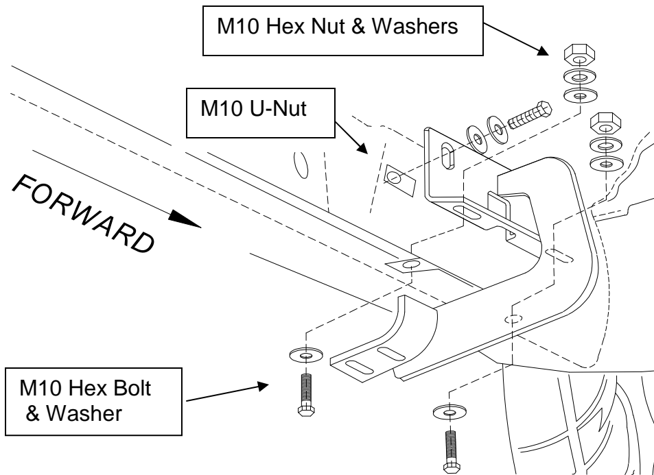
Figure 1. Driver Side – Front Bracket
