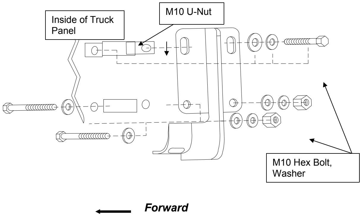
Figure 2. Passenger Side – Rear
