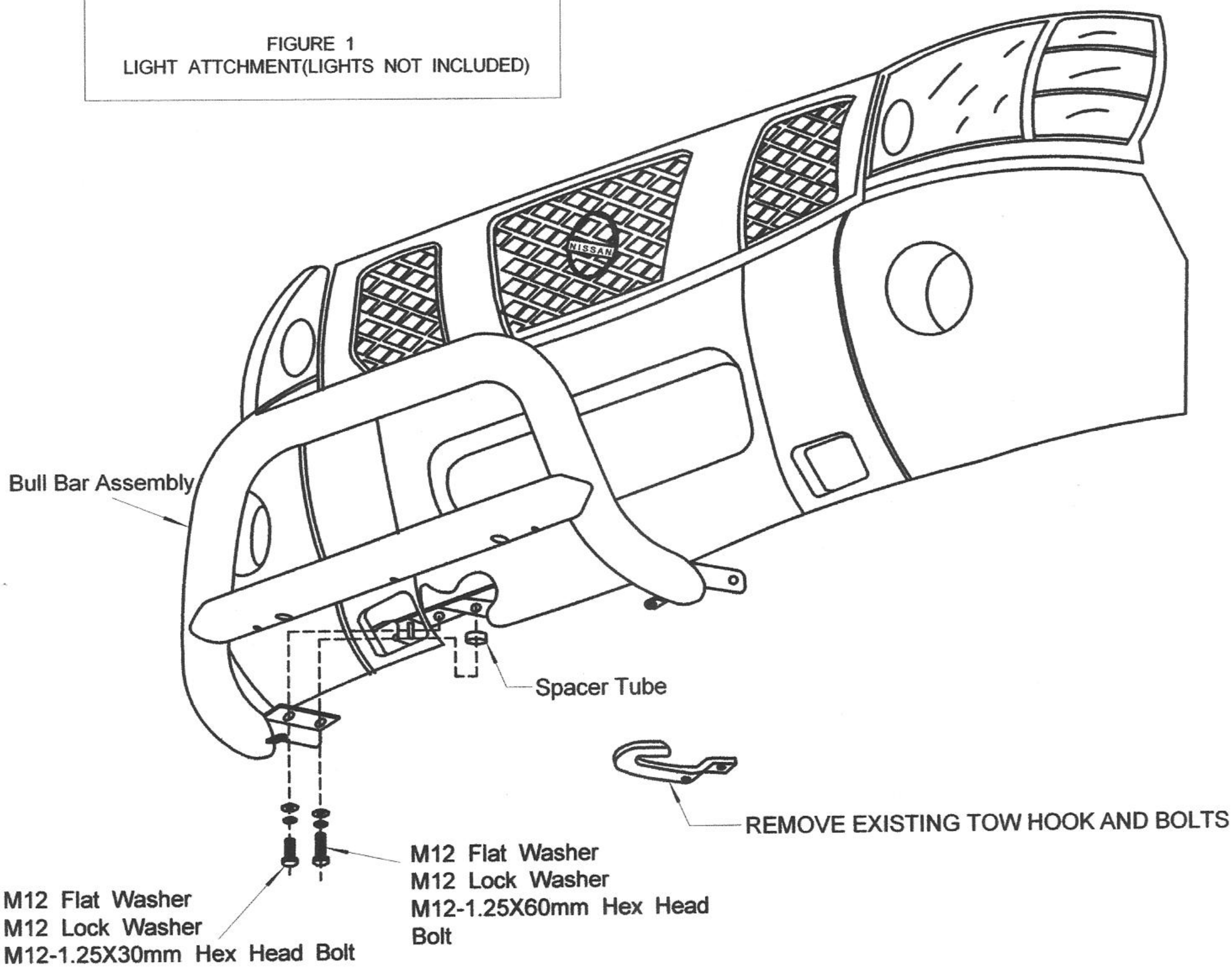
FIGURE 2 INSTALLATION OF PASSENGER SIDE, DRIVER SIDE OPPOSITE (SKID PLATE REMOVED FOR CLARITY.)
